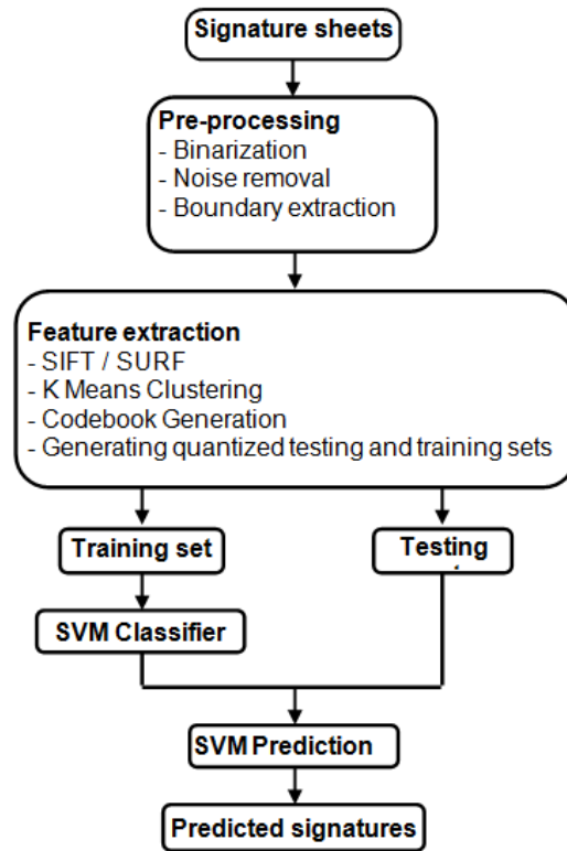
Fig. 1. Flow chart indicating boundary extraction procedure
