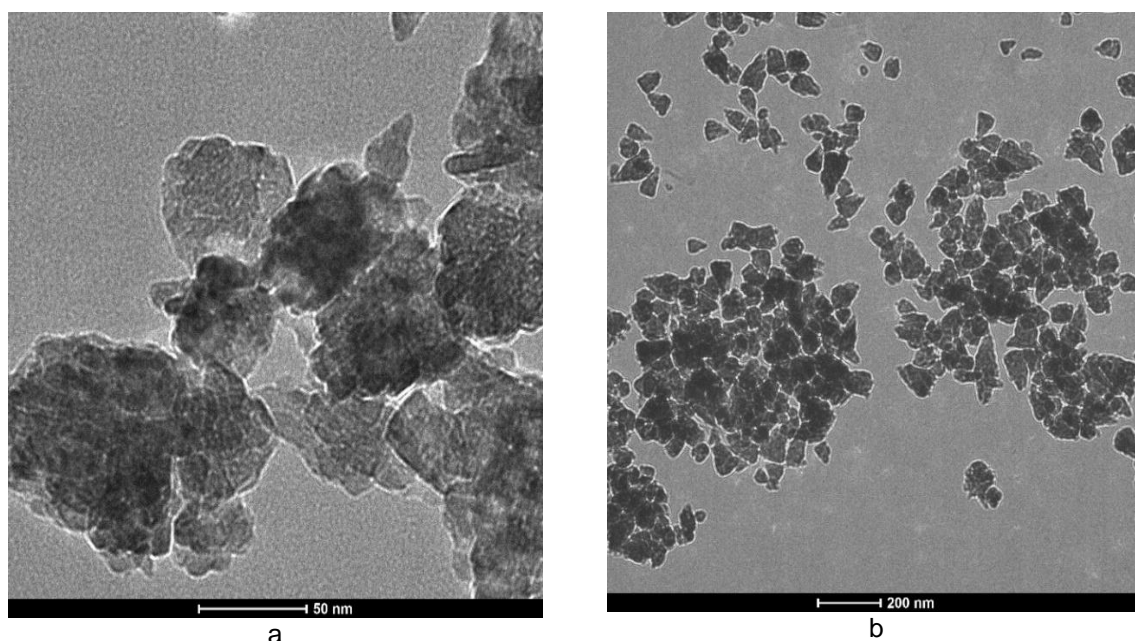
Fig. 3. TEM images of the fabricated nano composites
