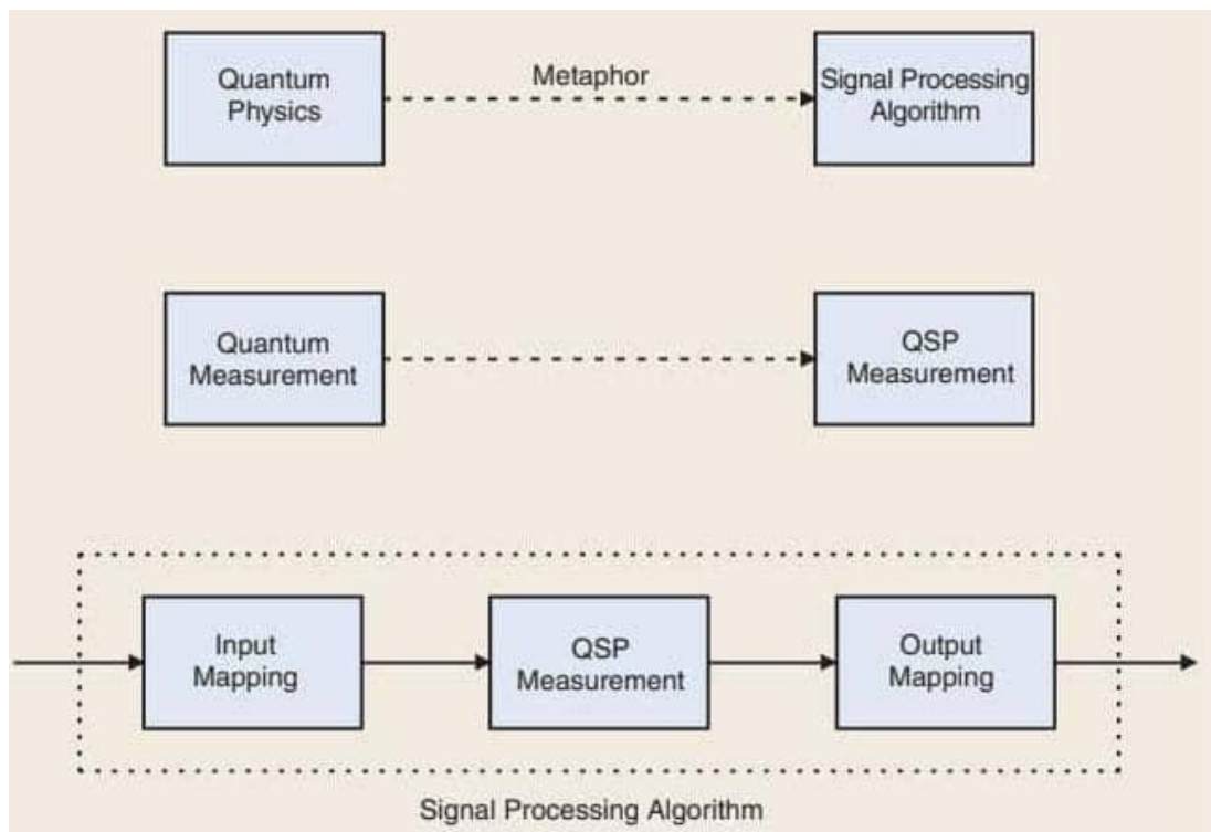
Fig. 1. Conceptual QSP measurement framework
