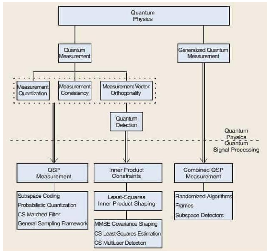
Fig. 2. QSP framework connected to quantum physics and relevant key results
