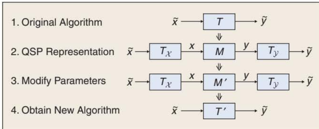
Fig. 4. Fundamental steps of QSP measurement for existing signal processing algorithms modification
