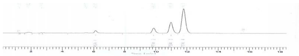
Fig. 9. Hydrolysis of artesunate in alkaline medium
