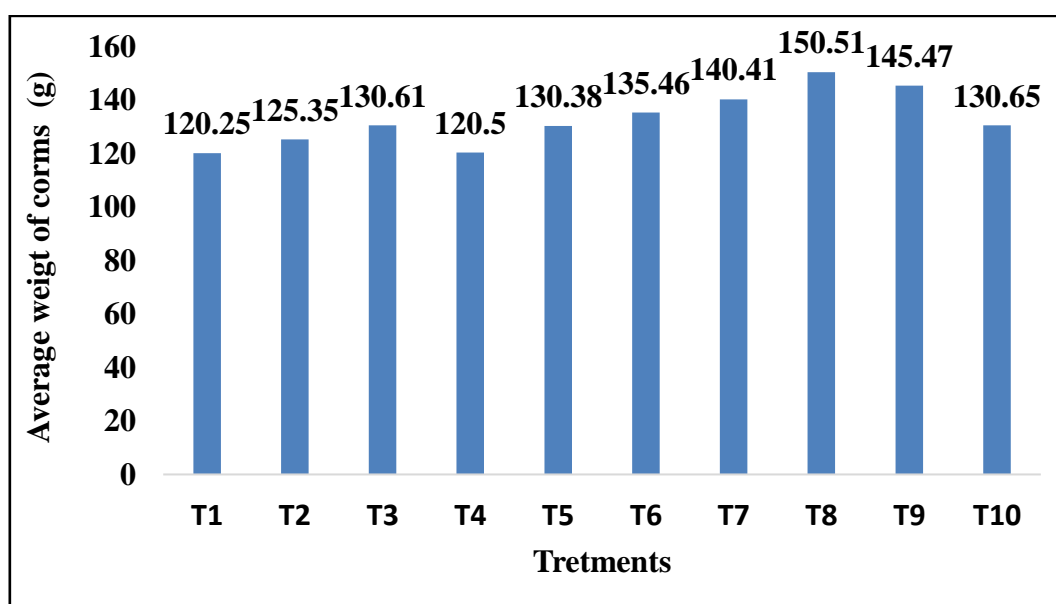
Fig. 1. Effect of various treatments of organic manures and inorganic fertilizers on average weight of corms(g) of gladiolus cv. Nova Lux
