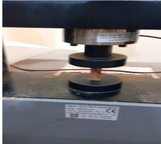
Fig. 2. Maximum Compressive Strength (MCS) parallel to grain test on a Universal Testing Machine
