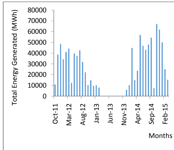
Fig. 7. Monthly total energy generated by the plant
