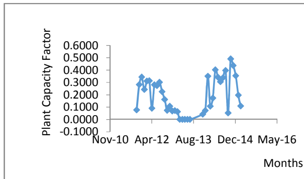
Fig. 4. Monthly plant capacity factor for the plant
