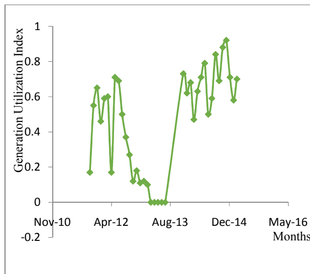
Fig. 3. Generation utilization index for the power plant
