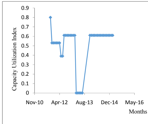
Fig. 2. Capacity utilization index for the power plant
