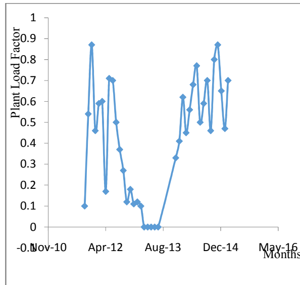
Fig. 1. Plant load factor for the power plant
