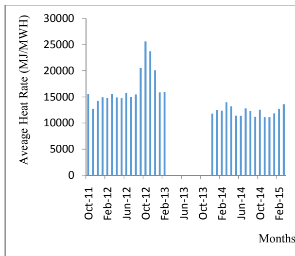
Fig. 6. Average heat rate of the power plant
